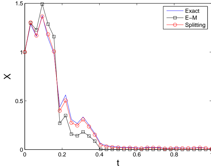
Figure 1: The plots of the exact solution (65), the approximate solutions for the linear problem (64) by the E-M method and the splitting method respectively with \Delta t = \frac{1}{2^5} .
