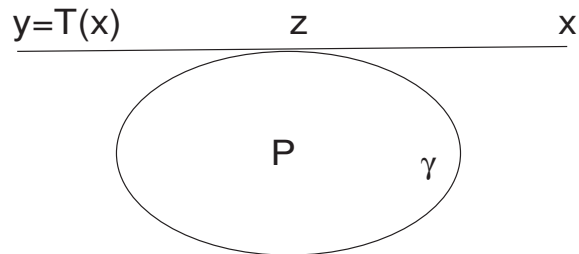
Figure 1: Defining the dual billiard map
