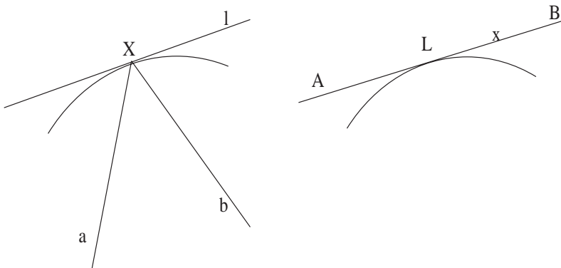
Figure 13: Duality between inner and outer billiards
