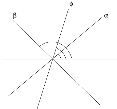
Figure 16: Harmonic quadruple of lines given by angles
