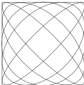
Figure 10: Ellipses inscribed into a square
