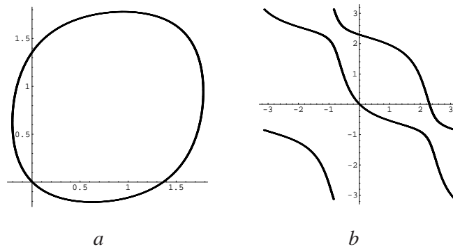
Figure 15: Two invariant curves (the right one consists of two components, the phase points “jump” from one component to the other)
