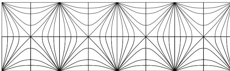
Figure 17: Level curves of the integral I in the (\alpha, p) -coordinates
