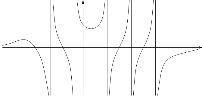
Figure 8: The graph of the function f(\lambda) for a time-like point x
