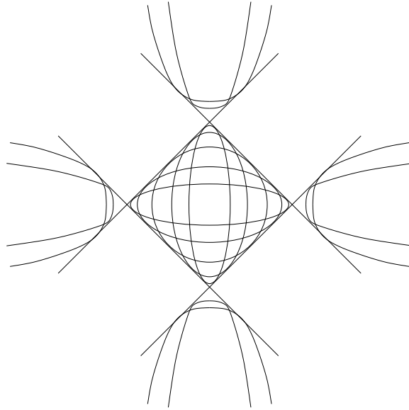
Figure 9: A pseudo-confocal family of conics
