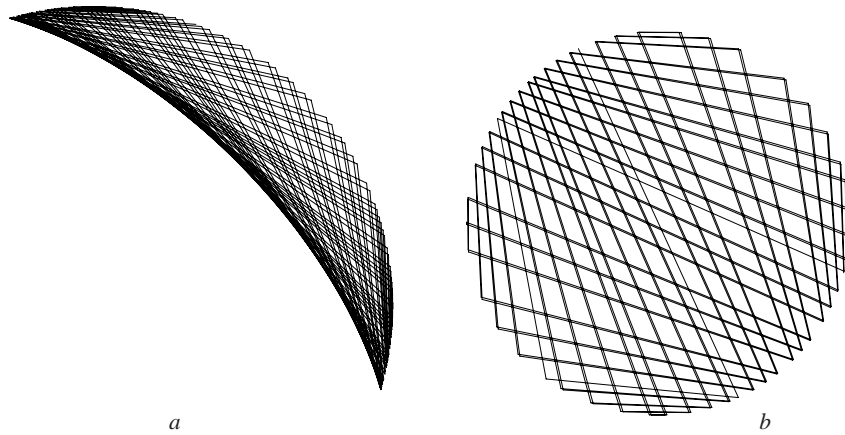
Figure 12: Two orbits consisting of 100 billiard segments: the lines containing the billiard segments on the left are tangent to an ellipse, and those on the right to a hyperbola
