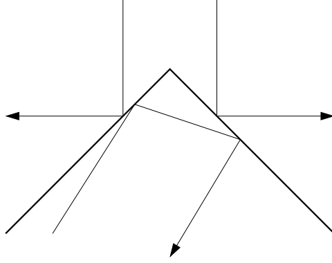
Figure 4: Euclidean billiard reflection in a right angle
