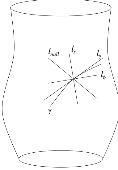
Figure 7: A quadruple of tangent lines on a surface of revolution
