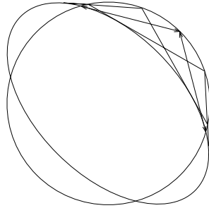
Figure 11: Two 4-periodic trajectories on the invariant curve with the rotation number 1/4 : one orbit is a self-intersecting quadrilateral, and the other one consists of two segments, traversed back and forth
