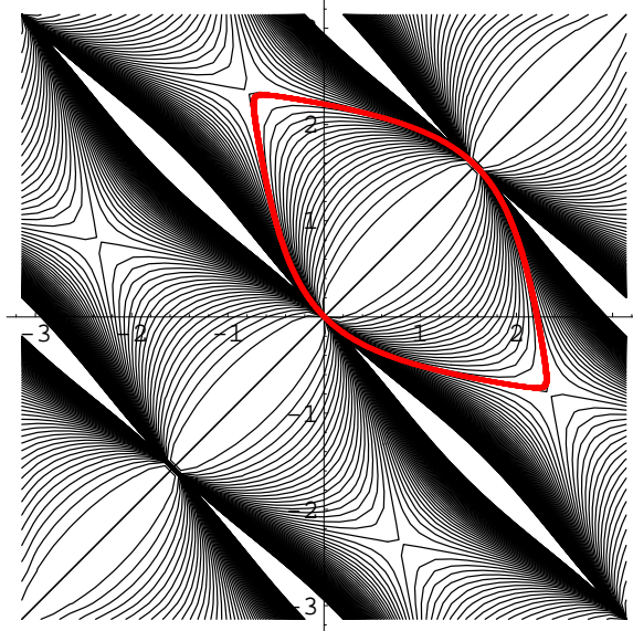
Figure 14: Level curves of the integral I in the (t_1, t_2) coordinates
