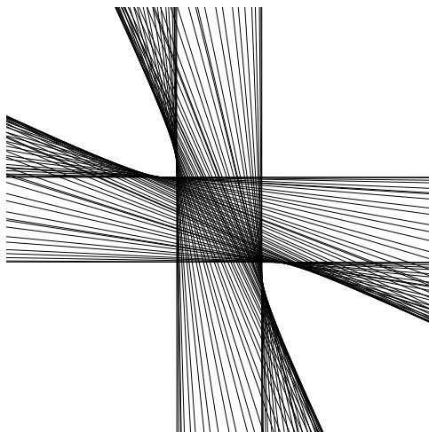
Figure 13: Extensions of billiard chords tangent to a hyperbola
