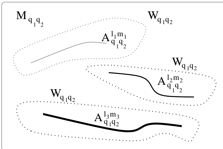
FIGURE 2. Coexistence of Countably Many Traveling Wave Submanifolds
