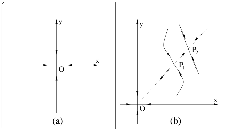
FIGURE 7. The Phase Portraits for the FitzHugh-Nagumo Equation: a) the local map has two fixed points (O is attracting, \infty is repelling); b) the local map has four fixed points (O and P_2 are attracting, P_1 is saddle, and \infty is repelling).
