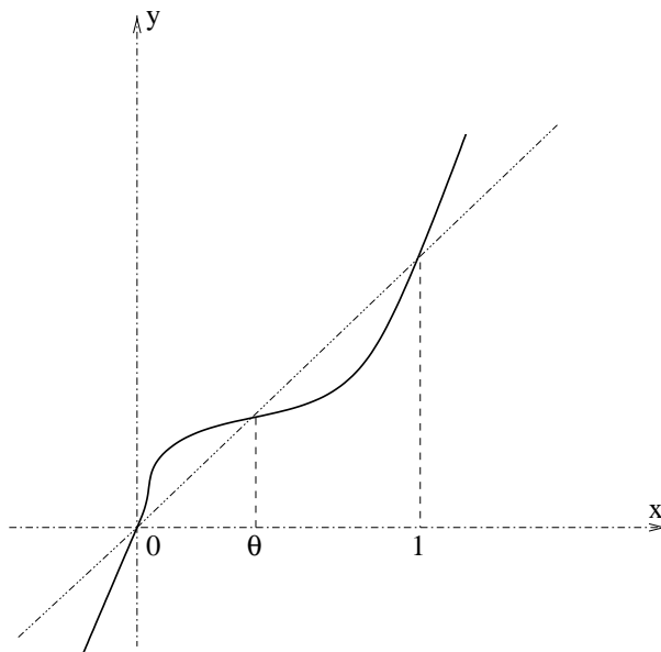
FIGURE 4. The Local Map for Huxley Equation ( \nu < 0 )
