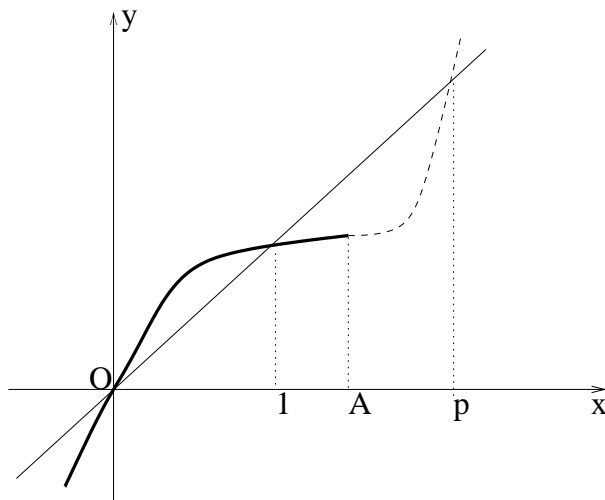
FIGURE 5. The Change of the Local Map for the KPP Equation
