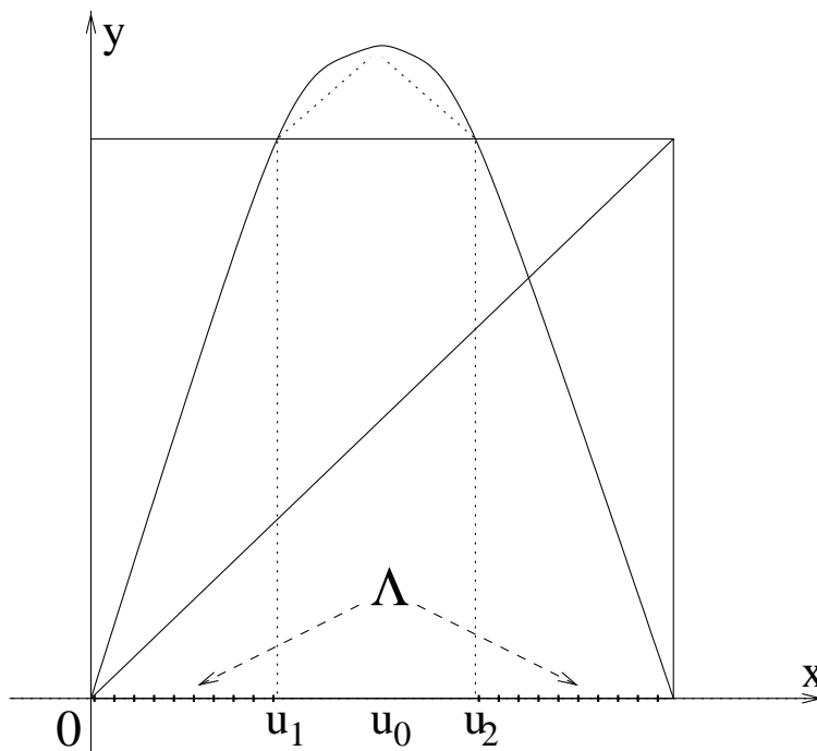
FIGURE 6. Expanding Local Map for the KPP Equation
