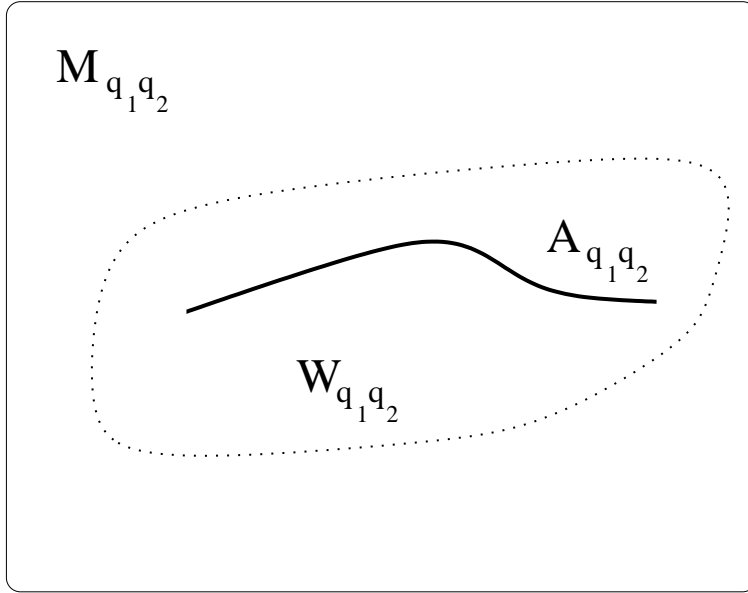
FIGURE 1. Stable Separatrix for a Traveling Wave Submanifold
