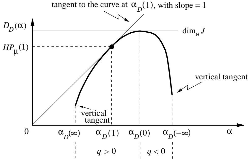
FIGURE 4. A typical graph of the function \mathcal{D}_D(\alpha) .
