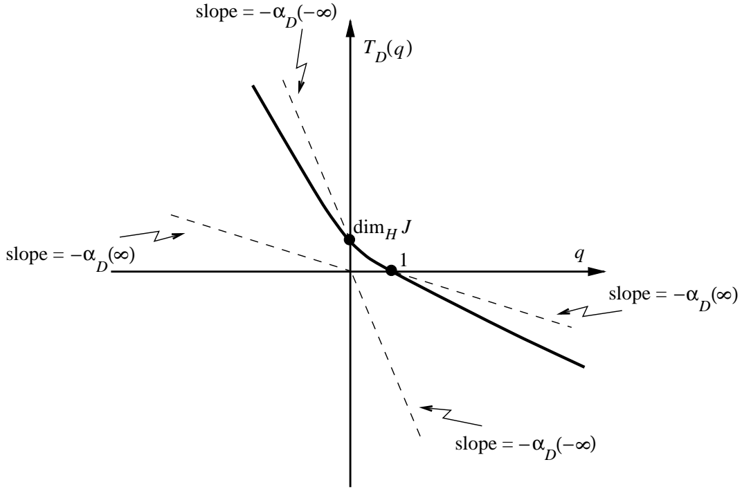
FIGURE 3. A typical graph of the function T_D(q) .
