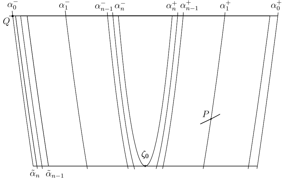
FIGURE 1. The rectangle R and the curves \{\tilde{\alpha}_n\} , \{\alpha_n^+\} , \{\alpha_n^-\} . The \{\tilde{\alpha}_n\} accumulate on the left stable side of R . Both \{\alpha_n^+\} and \{\alpha_n^-\} accumulate on the parabola in W^s(Q) containing the point of tangency \zeta_0 near (0, 0) .
