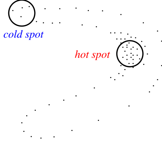
FIGURE 1. HOT AND COLD SPOTS ON AN ATTRACTOR
