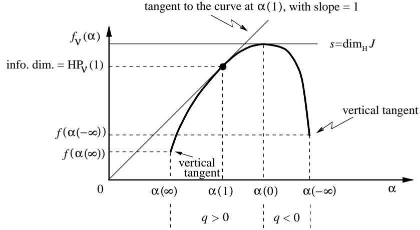
FIGURE 2B) f_\nu(\alpha)
