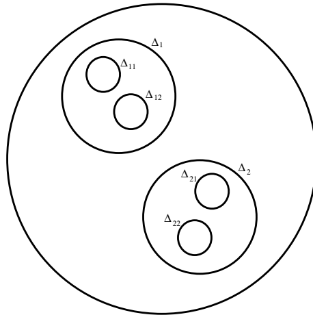
FIGURE 3. MORAN GEOMETRIC CONSTRUCTION WITH DISJOINT BASIC SETS
