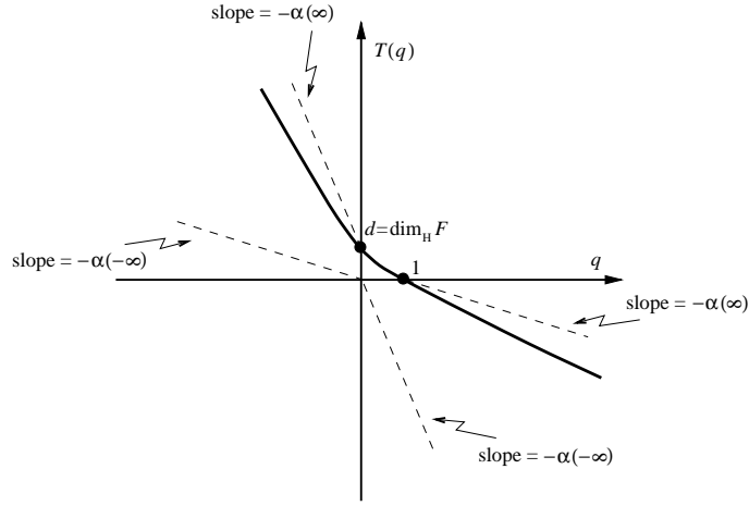
FIGURE 3A GRAPH OF T(q)
