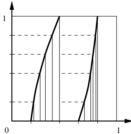
FIGURE 2B) A ONE-DIMENSIONAL MARKOV MAP
