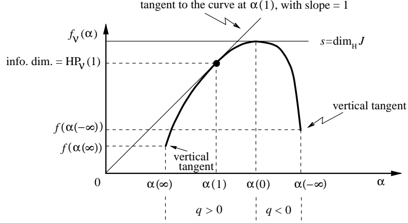
FIGURE 3B GRAPH OF f_\nu(\alpha)
