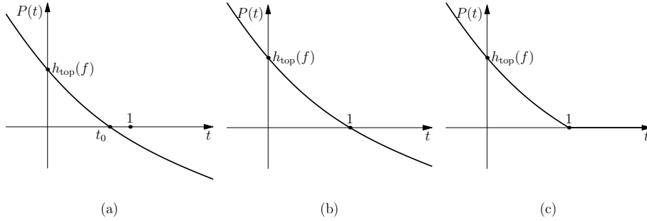
FIGURE 1.1. The pressure function for (a) typical hyperbolic sets; (b) a hyperbolic attractor; (c) a non-uniformly hyperbolic map with a phase transition.
