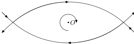
FIGURE 1. Separatrices
