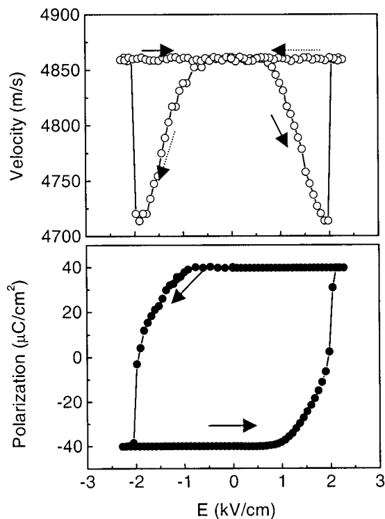
FIG. 2. Velocity-electric field loop and polarization-electric field loop. The longitudinal velocity is measured in [111] under an electric field also in [111].
